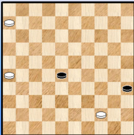
Diagram 23A
