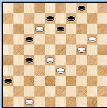
Diagram 1C 28-22 !
