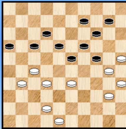
Diagram 10 Waz
