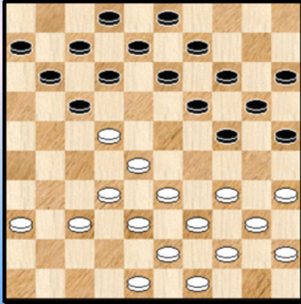
Diagram 1 36-31 ?
