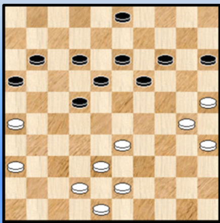
Diagram 4 19-23 ?
