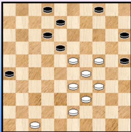
Diagram 3 26-31 ?
