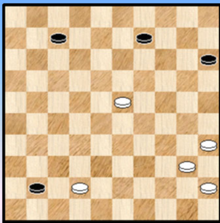
Diagram 7A Waz
