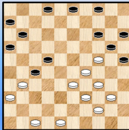
Diagram 4C Waz
