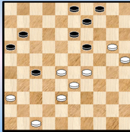
Diagram 1A 28-22 !
