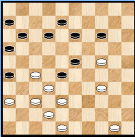
Diagram 21 13-18 ?
