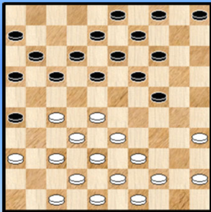
Diagram 16 44-40 ?
