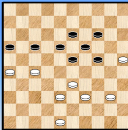
Diagram 9 48-42 ?
