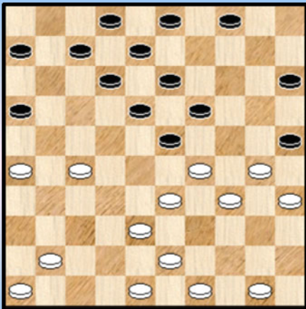
Ger Stam 12-17 ?
