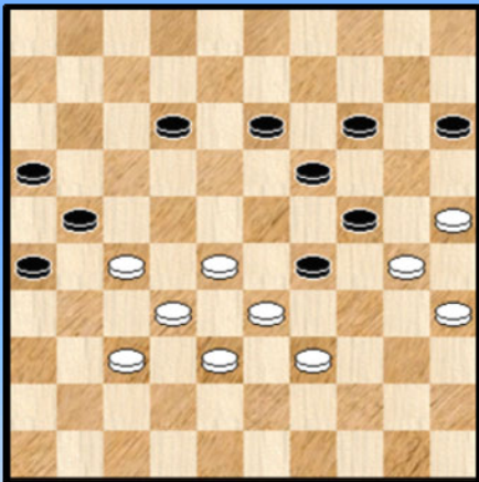
Diagram 2 27-22 ?
