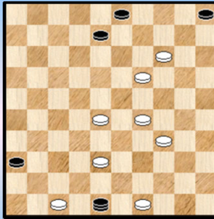
Diagram 43B 02-08 ?
