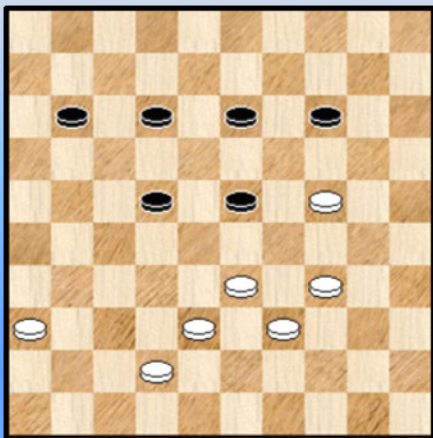
Diagram 23 42-37 ?
