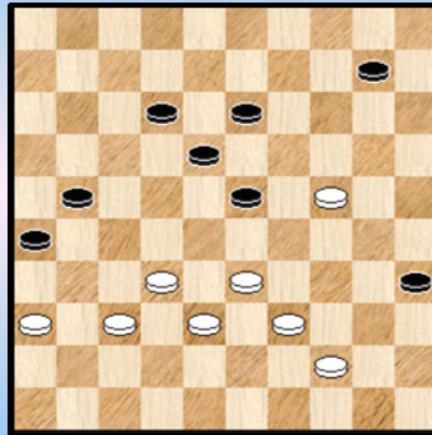
Diagram 3A 23-29 ?
