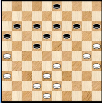
Diagram 1 19-23 ?
