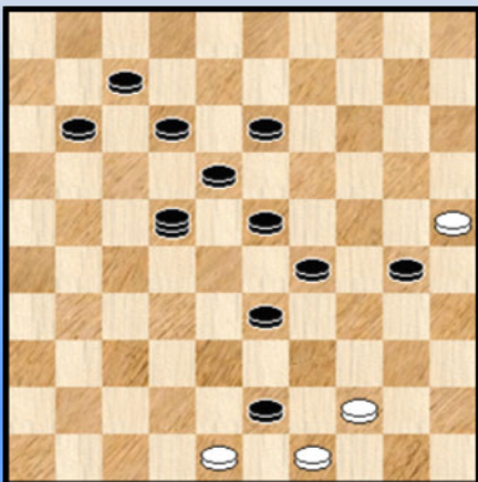
Diagram 13A
