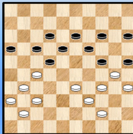
Diagram 3 37-32 ?
