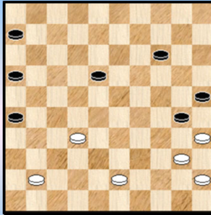
Diagram 7A
