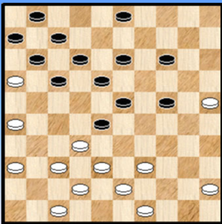
Diagram 5 24-29 ?
