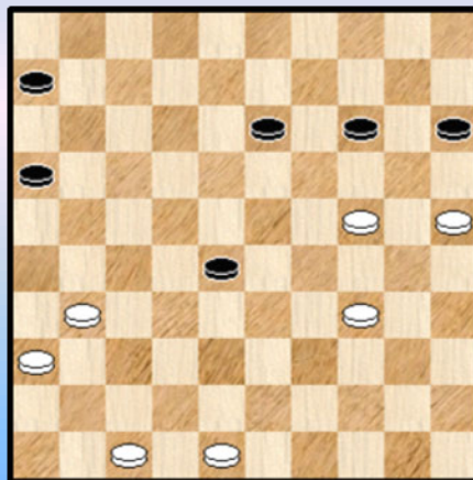
Diagram 3J Waz
