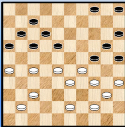
Diagram 1 37-32 ?
