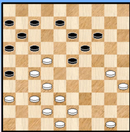
Diagram 20 43-39 ?
