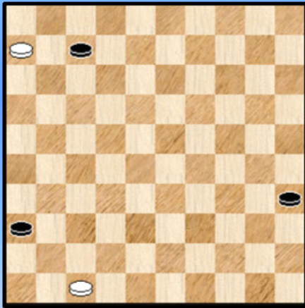
Diagram 22A Waz
