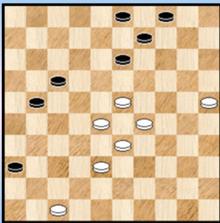
Diagram 1B 28-22 !
